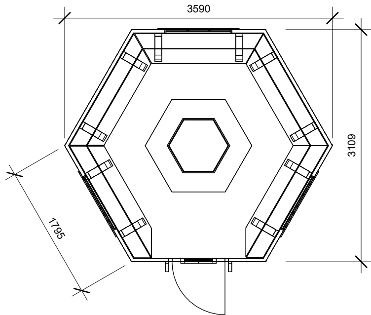
PLAN (1:50)
