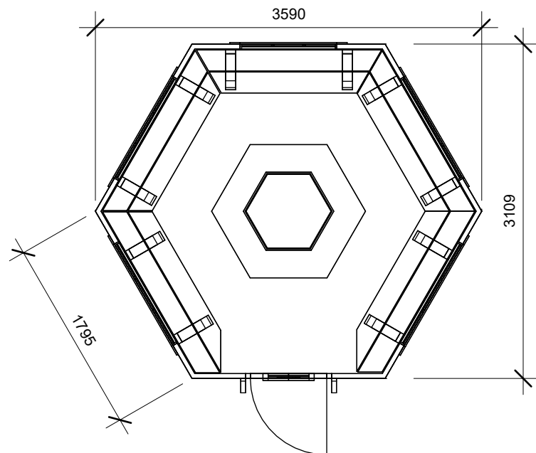
PLAN (1:50)
